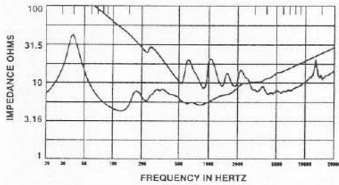
FIGURE 2 — MTH-2.5/64B Impedance vs. Frequency
